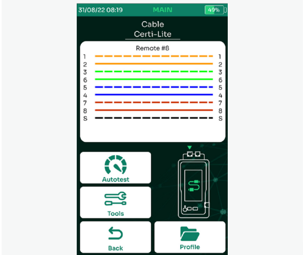
Figure 5 - Wiremap with Remote ID#8 Identified
