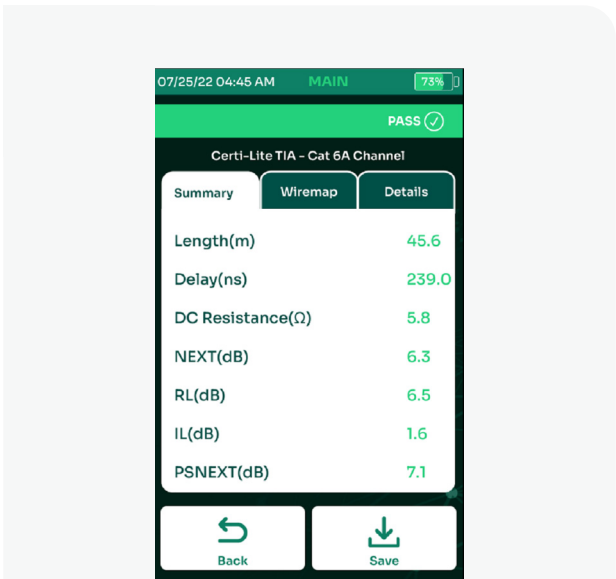
Figure 4 - Certi-Lite Autotest result can be obtained with Remote IDs. Click on Details tab to drill into each test result. Test Results can be stored in tester memory for later upload to the included PC based TestDataPro, or immediately with the included TestDataPro Cloud via wired or wireless network connection.
